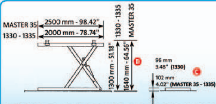
EH ELECTROHYDRAULIC
