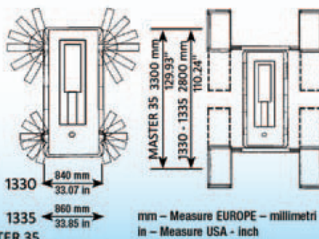
PH PNEUMOHYDRAULIC
